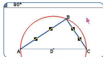
Dynamic geometry
